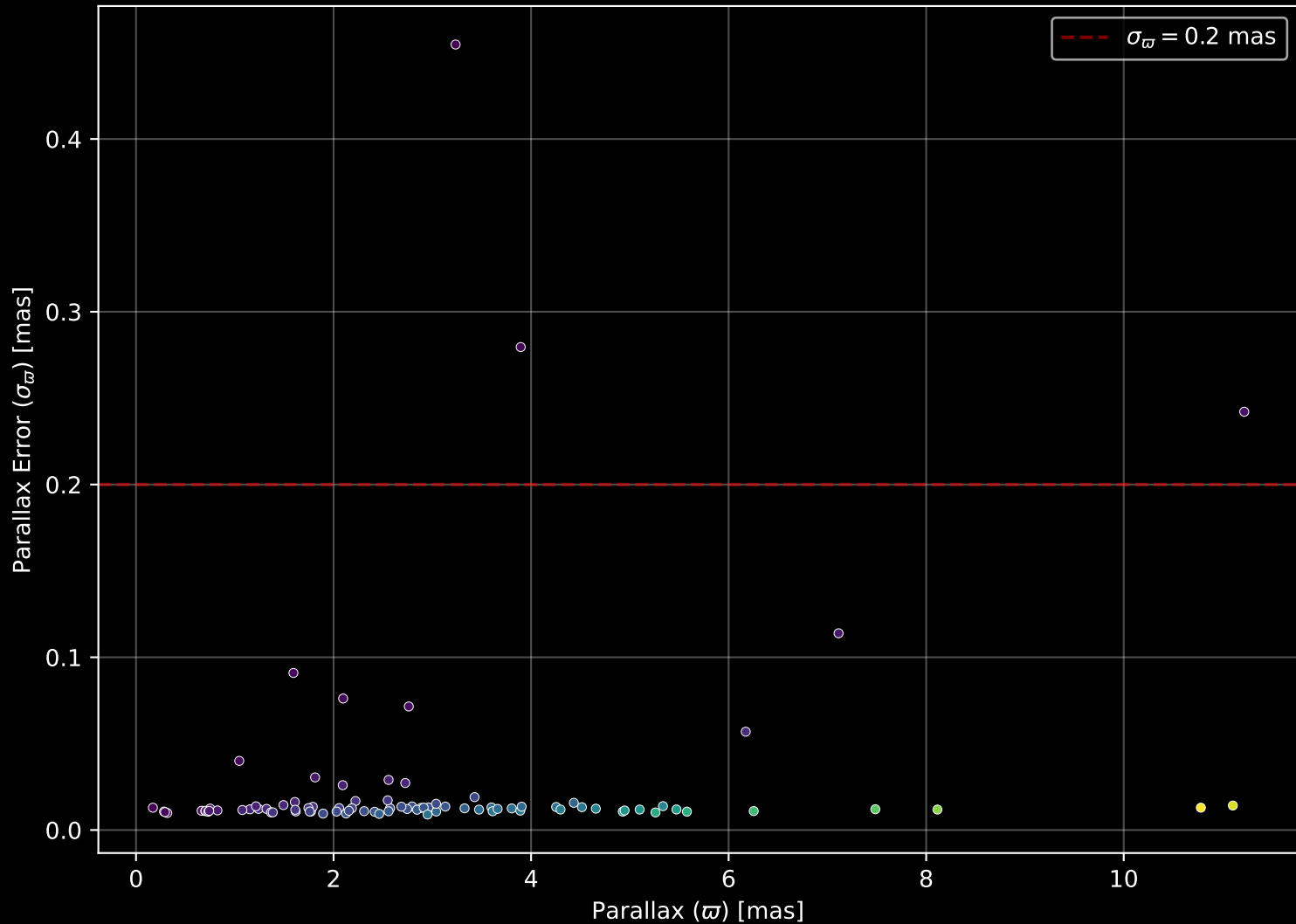
GALAH DR4 Field: [7179] Parallax Quality (n= 90)
