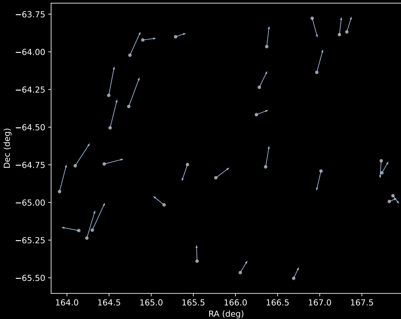
GALAH DR4 Cluster 1 Proper Motion Vectors (n=31)
