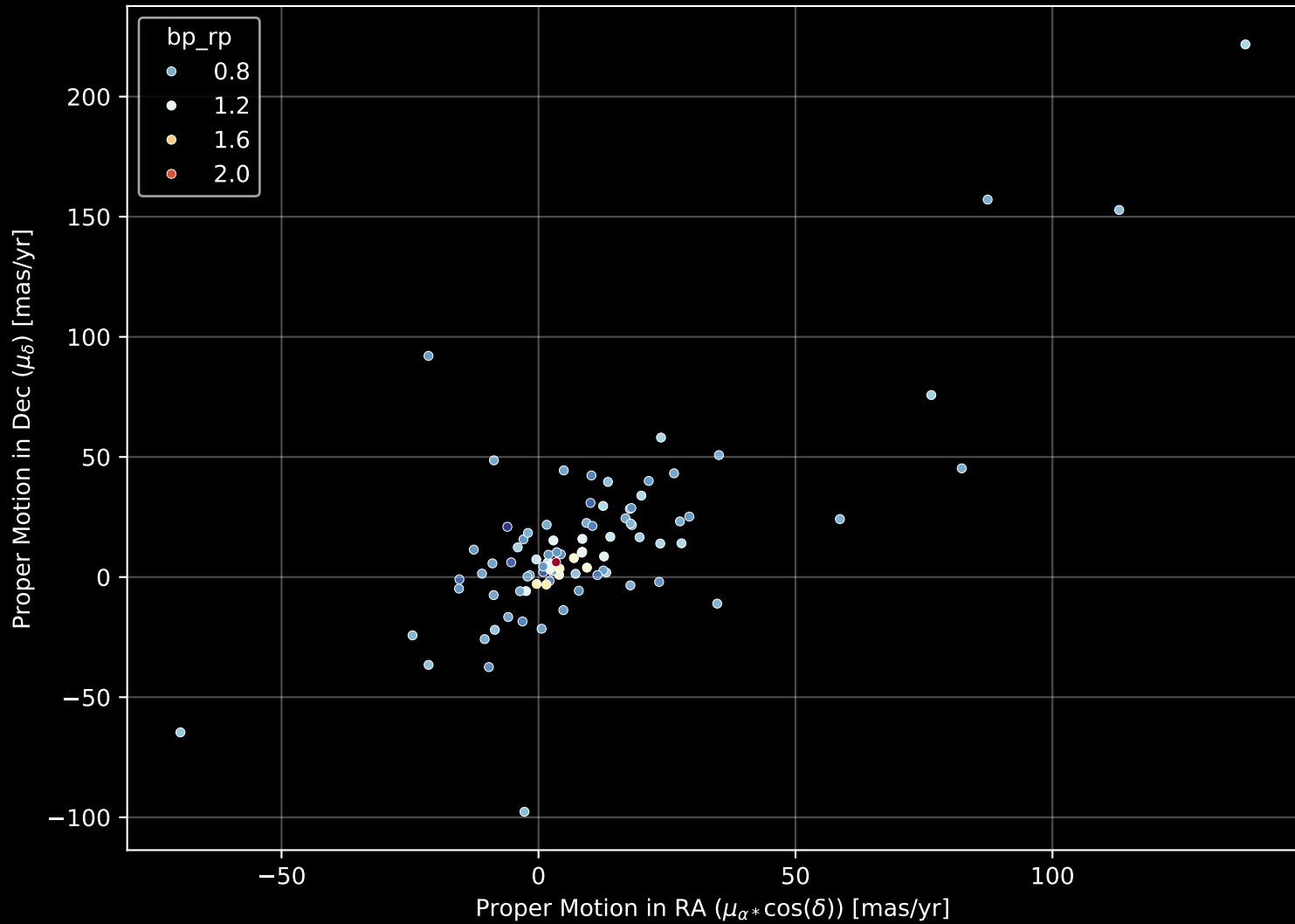
GALAH DR4 Field: [7179] Proper Motion Diagram (n= 90)
