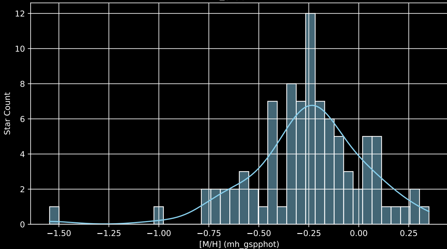
GALAH DR4 Field: [7179] [M/H] (mh_gspphot) (n= 90)
