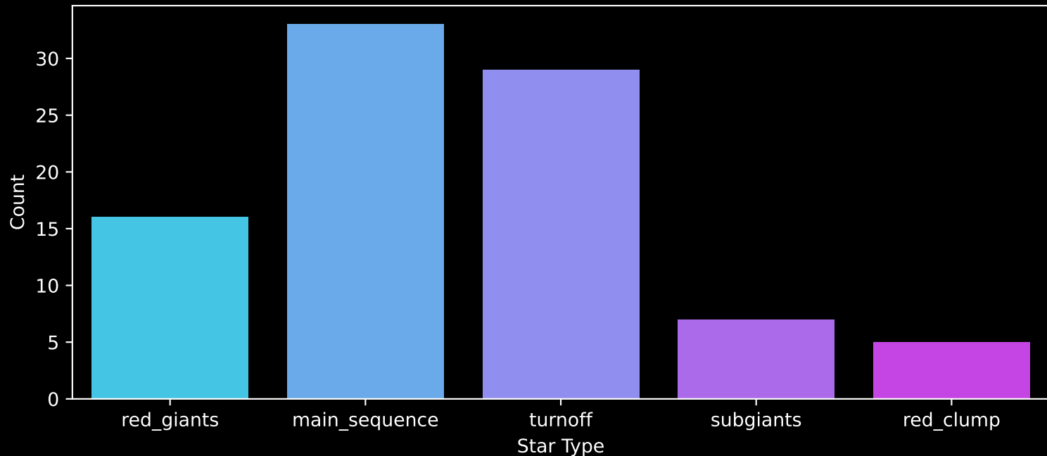
GALAH DR4 Field: [7179] Count plot of Star Type
