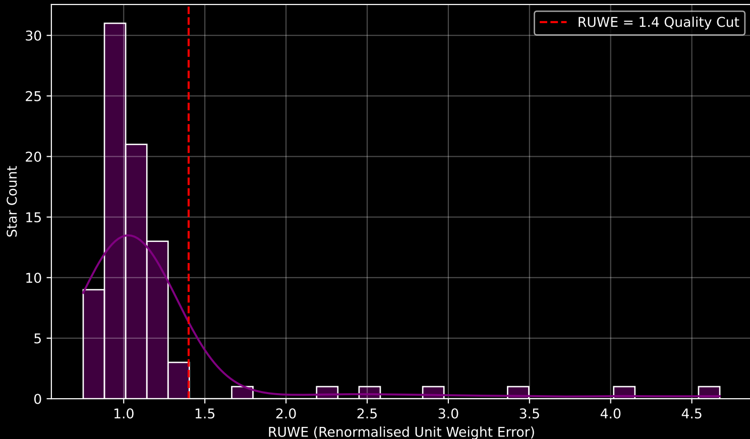
GALAH DR4 Field [7179] RUWE Distribution (n= 84)
